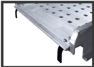
TYPE F - FLUSH HOOK Steel hooks lock onto the truck bed provided flush-type direct entry
