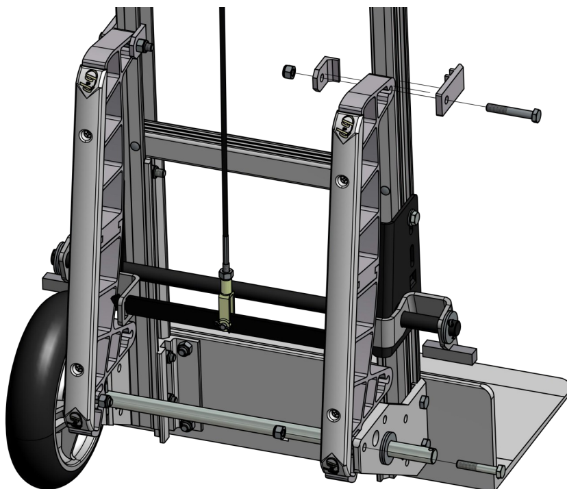
Installation with 8" wheels, with or without tread brakes. (Flip stair climber orientation)
